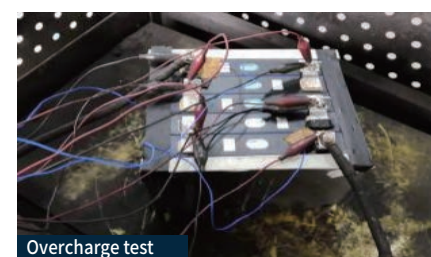
Overcharge test
