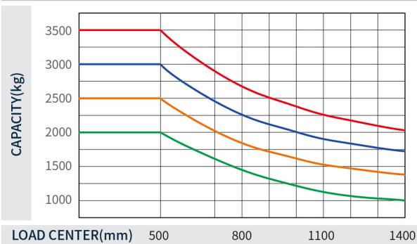
Load curve
